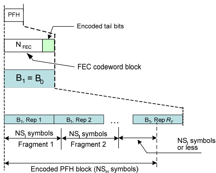
Figure 8-13 – Generation of the encoded PFH block
