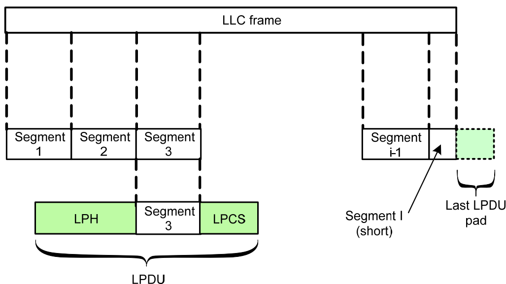
Figure 9-7 – Generation of LPDUs from LLC frames
