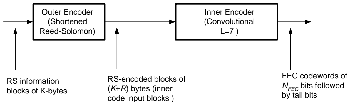
Figure 8-7 – FEC encoder
